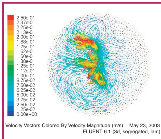
Velocity plots generated using the new Chemineer Clean Sweep Mixer
